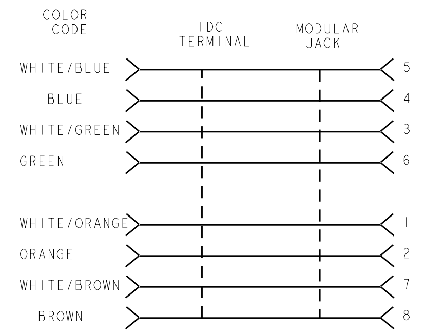
ELECTRICAL SCHEMATIC T568B
