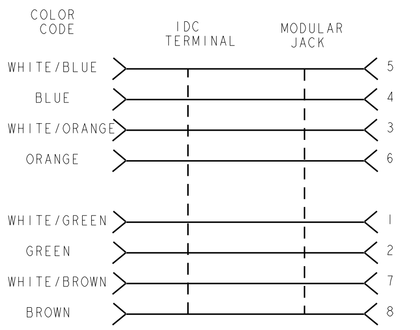
ELECTRICAL SCHEMATIC T568A
